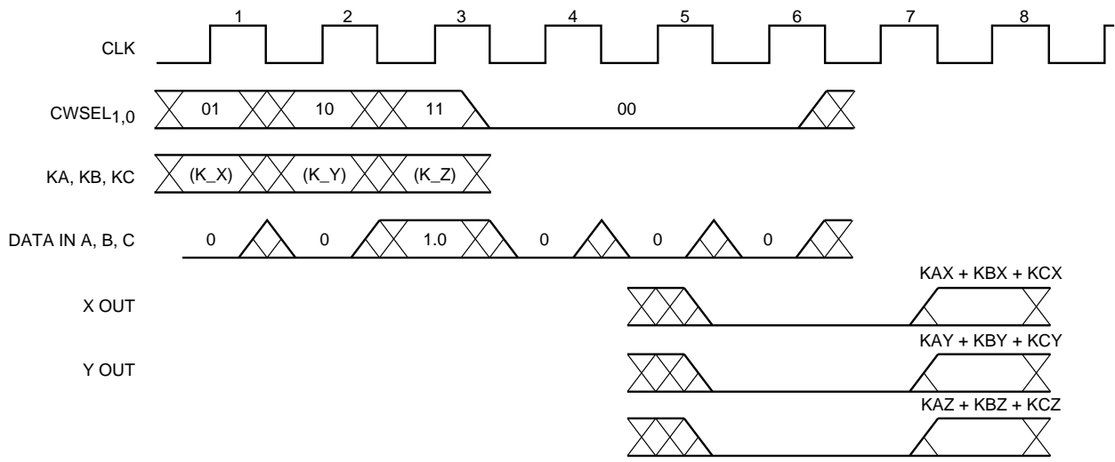
Figure 1. Impulse Response
